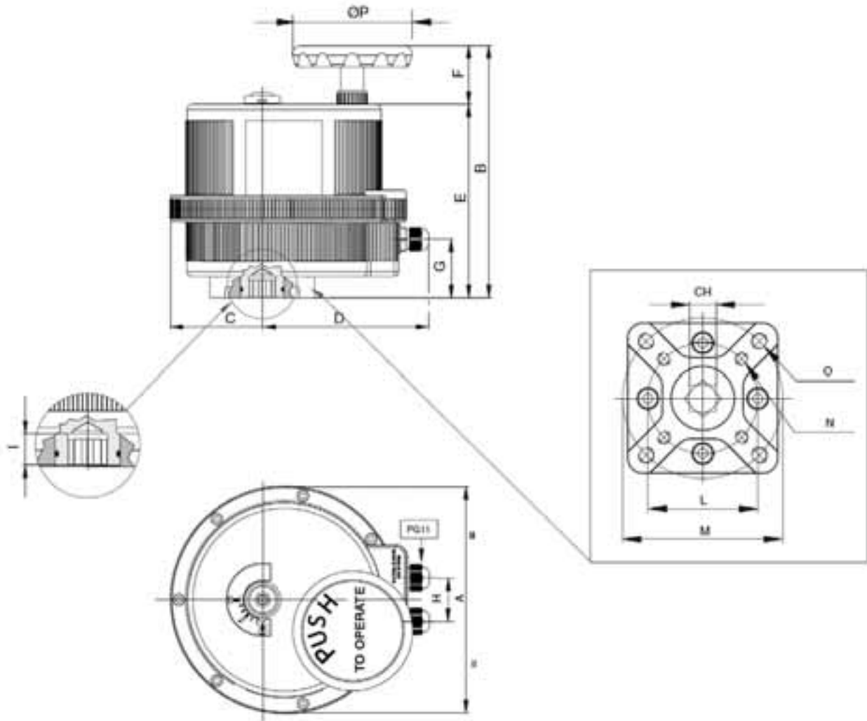
DIMENSIONS (inches)
