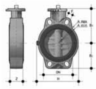
DIMENSIONS (inches)
