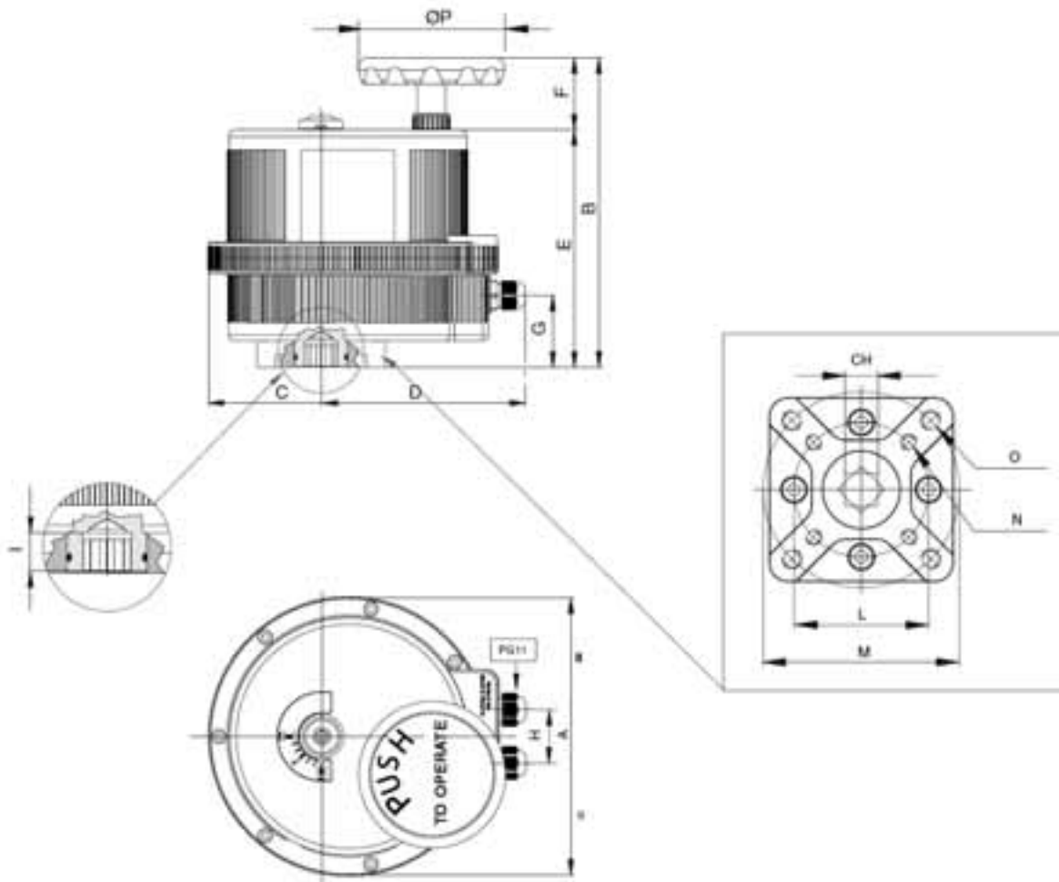
DIMENSIONS (inches)
