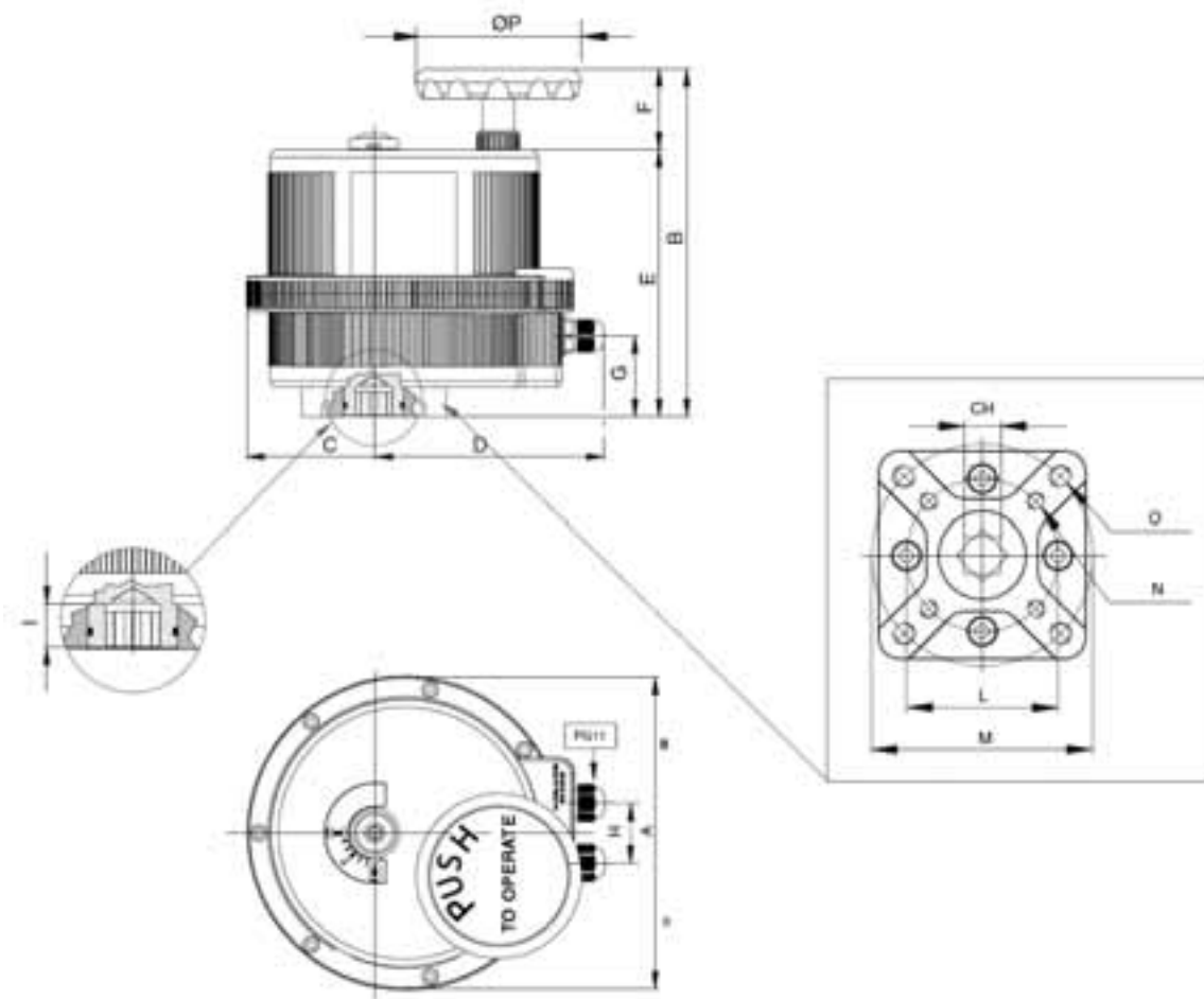
DIMENSIONS (INCHES)
