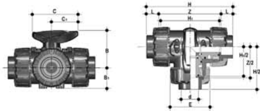
DIMENSIONS (inches)
